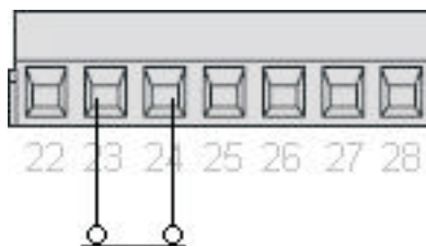
PHOTOCELL CONNECTION ON OPENING (Microswitch n° 4 OFF)
